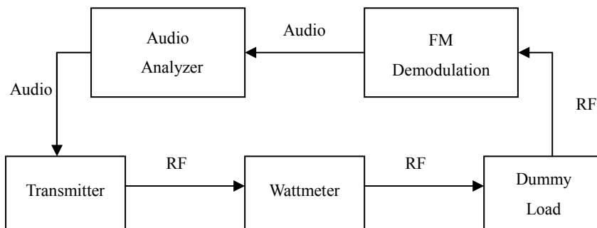
Figure 5-1 connecting for audio analyse
