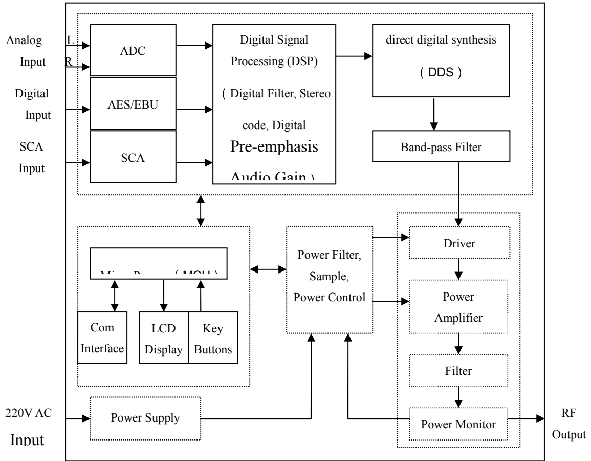
Figure 3-1 CZH618F-1000C transmitter structure and function
